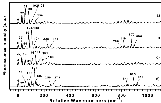
Figure 10. SVLF spectra of the 2HDPM A origin (a), +31 \text{cm}^{-1} (b), +42 \text{cm}^{-1} (c), and +62 \text{cm}^{-1} (d) bands.
