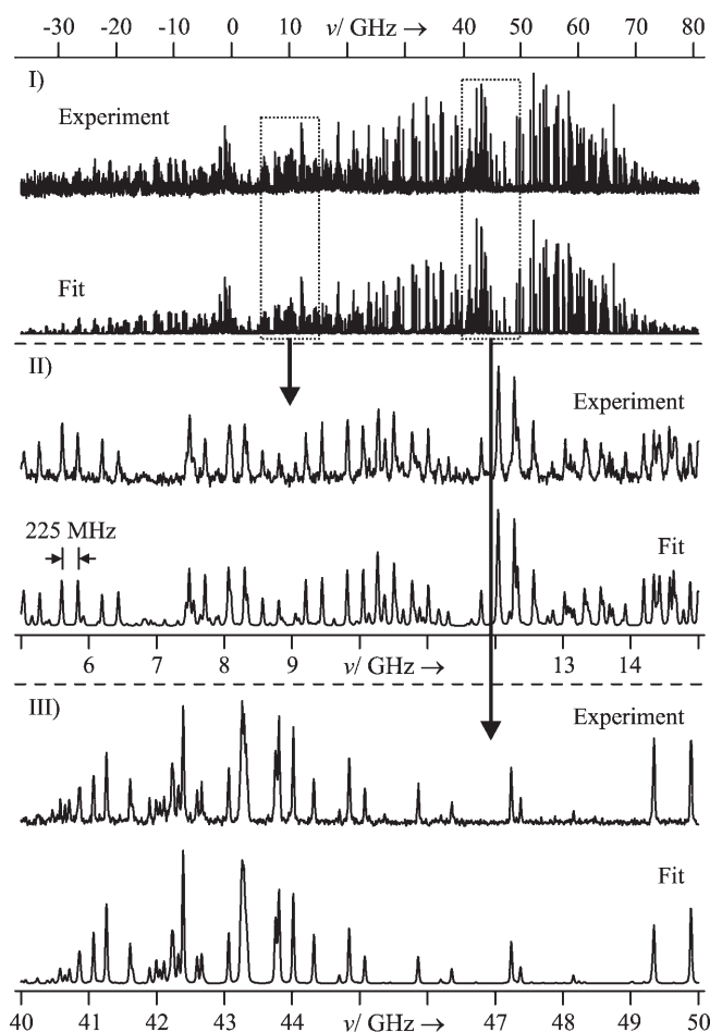
Figure 4. Experimental and fitted spectra of (1,2,4), (1,2,6) and (1,2,3,4) deuterated resorcinol B. I) Full spectra. The zero in the frequency scale corresponds to the origin of the (1,2,4) isotopomer. II) 10 GHz zoom-in of the part belonging to the (1,2,4) and (1,2,6) isotopomers. A small splitting of 225 MHz between these two bands is also shown. III) 10 GHz zoom-in of the origin vicinity of the (1,2,3,4) species.
