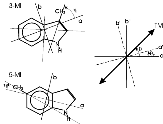
FIG. 1. Definition of \eta , the angle between the internal rotation axis and the principal a -axis, for 3-methylindole and 5-methylindole (left panel). In the right panel the transition moment angle \theta and the axis reorientation angle \theta_T are defined. Angles measured in counterclockwise sense are taken to be positive. a'' and b'' are the principal axes in the ground state, a' and b' are the principal axes in the excited state. The c axes are perpendicular to the indole frame.
