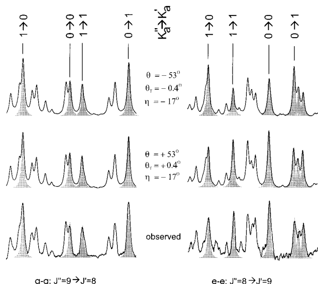
FIG. 6. Parts of the 0a_1-0a_1 and 0e-0e spectrum of 5-methylindole. The lower panels show the observed spectrum. The middle panels show simulations, using positive values for the transition moment and axis reorientation angle. A simultaneous change of sign of \theta and \theta_T does not affect the line positions but yields different intensities for the 0e-0e transitions, as can be seen from the upper panels.
