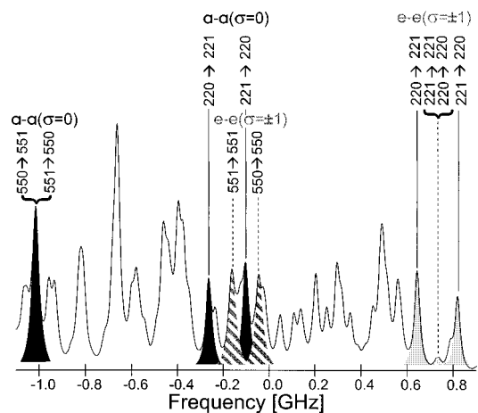
FIG. 3. Effect of internal rotation on a -type transitions in the Q -branch of 3-methylindole. Upper panel: e levels with high J, K_a value are split by FW_{0e}^{(1)} \rho_a K_a . The width of the arrows corresponds (approximately) to the strength of the transitions; the 0e - 0e transitions show a change from “normally allowed” transitions ( \Delta K_c = \pm 1 ) for low K_a values, where the asymmetry splitting is large, to anomalous transitions ( \Delta K_c = 0 ) for high K_a values, where the asymmetry splitting is much smaller. This is also illustrated by part of the experimental spectrum of 3-methylindole (lower panel), where the corresponding transitions are marked.
