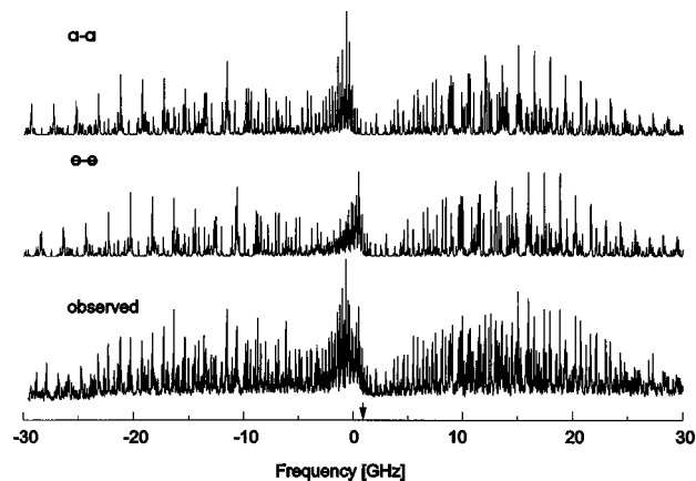
FIG. 4. Experimental spectrum of 3-methylindole (lower panel) together with simulations of the 0a_1-0a_1 and 0e-0e transitions (upper two panels). The 0a_1-0a_1 origin (0 on the scale of the figure) is located at 34\,874.69(1)\text{ cm}^{-1} . The origin of the 0e-0e band is indicated by the arrow.
