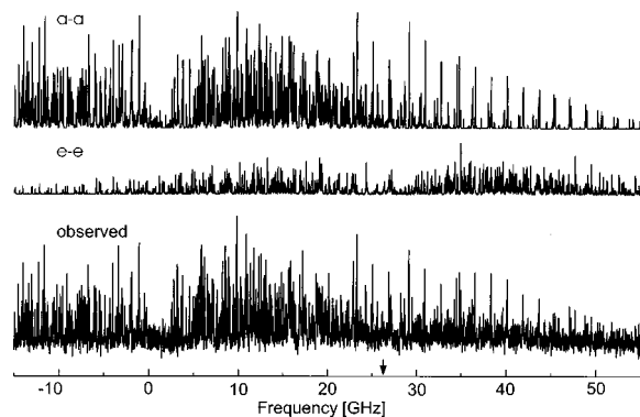
FIG. 5. Experimental spectrum of 5-methylindole (lower panel) together with simulations of the 0a_1-0a_1 and 0e-0e transitions (upper two panels). The 0a_1-0a_1 origin (0 on the scale of the figure) is located at 34\,355.915(12)\text{ cm}^{-1} . The origin of the 0e-0e band is indicated by the arrow.
