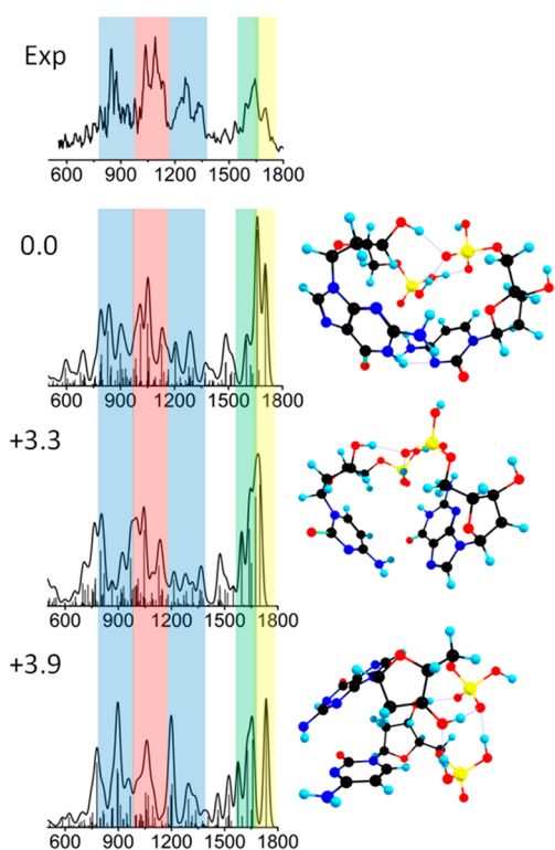
Figure 4. Experimental spectrum of [dGMP-dCMP-H] 1- plotted with the three lowest energy calculated spectra. \Delta G energies are given in kcal/mol and are relative to the minimum energy structure.
