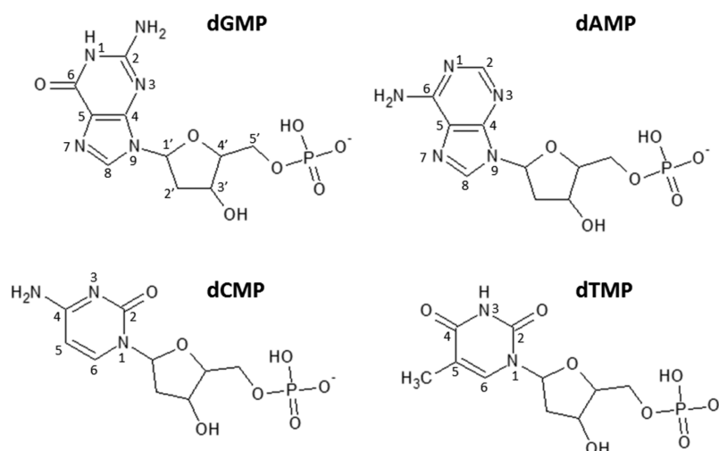
Figure 1. Molecular structures for the four 2'-deoxynucleotide-5'-monophosphate anions.
