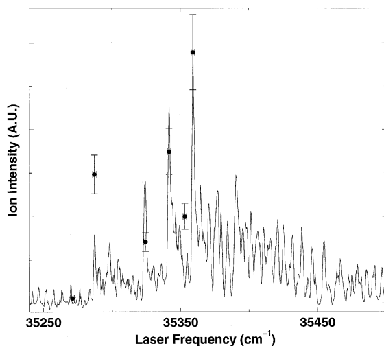
Fig. 4. The spectrum of vibrationally deexcited metastable CO molecules is sampled on top of, and in between a number of bandheads (indicated by the circles with error bars). For comparison, the b(v = 0) \leftarrow a(v = 0) spectrum recorded for the scattering of CO a^3\Pi(v = 0) [16,17] is indicated by the solid line.
