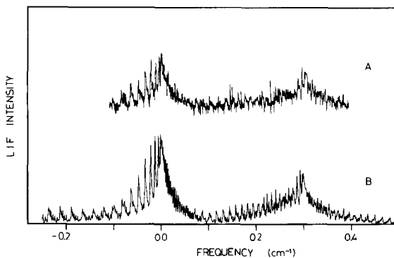
Fig. 7. Experimentally observed (a) and simulated (b) high-resolution LIF spectrum of the origin of the 211 \text{cm}^{-1} blue-shifted TPA-Ar complex at 29731.2 \text{cm}^{-1} . The simulated TPA-Ar spectrum is for a van der Waals complex that is a symmetric top, i.e. a vdW complex in which the Ar atom is sitting on the c -axis. In the simulation the same rotational temperature (4.0 K), the same lineshape (Lorentzian, 40 MHz fwhm) and the same values for C'' and \Delta C were taken as found for TPA. The simulated spectrum is for B'' = 280 \pm 5 MHz and \Delta B = -8.5 \pm 0.5 MHz. As now \Delta B is negative, the R-branch has a band head and the Q-branch degrades to the red.
